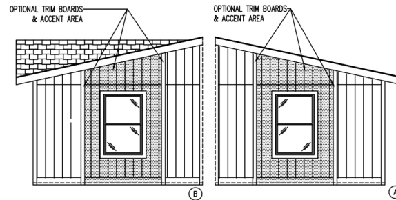
OPTIONAL FRONT ENDWALLS WITH ACCENT AREAS
